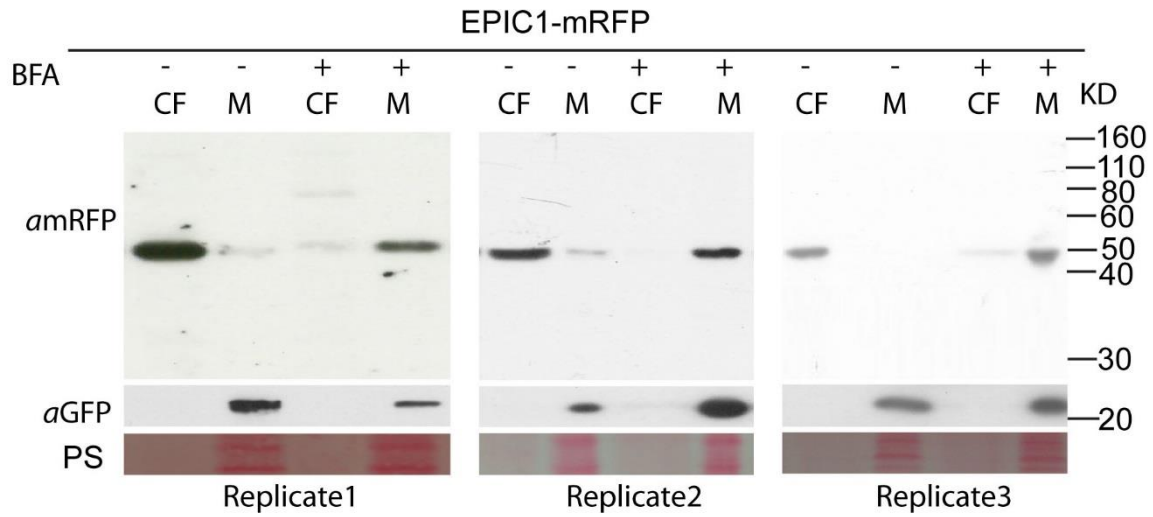
FIG S1 Analysis of the efficacy of BFA treatments on the samples of the transformant expressing EPIC1-mRFP (9) used for the LC-MS/MS assay. Immunoblotting was carried out to show BFA treatment (+) blocks secretion of EPIC1-mRFP by the conventional secretory pathway in three independent biological replicates. Green fluorescent protein was used as marker of cytoplasmic protein and showed that the CF preparation was not detectably contaminated with cellular protein.
