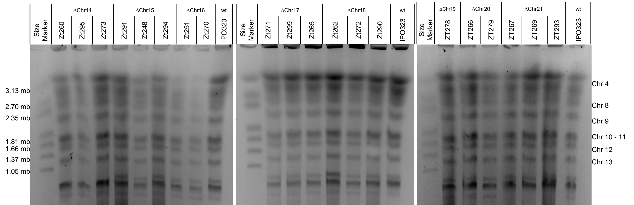
FIG S2 Pulsed-field gel electrophoresis for midsize core chromosomes of Z. tritici . Pictures of three pulsed-field gel electrophoresis gels for all strains used in this study. Size marker: Hansenula wingei chromosomes
