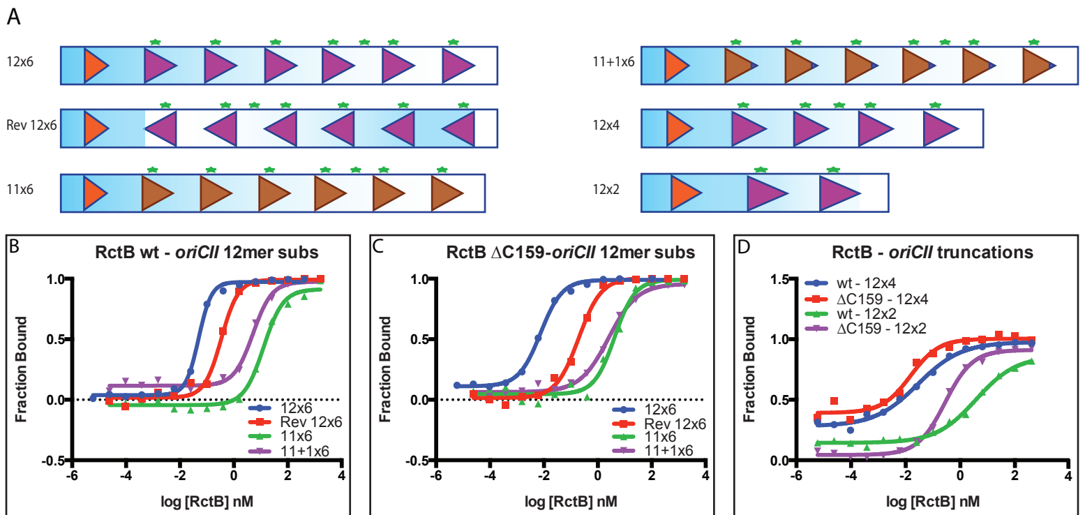
Figure S4 - 12-mer substitutions and deletions reduce RctB binding affinity and/or cooperativity
