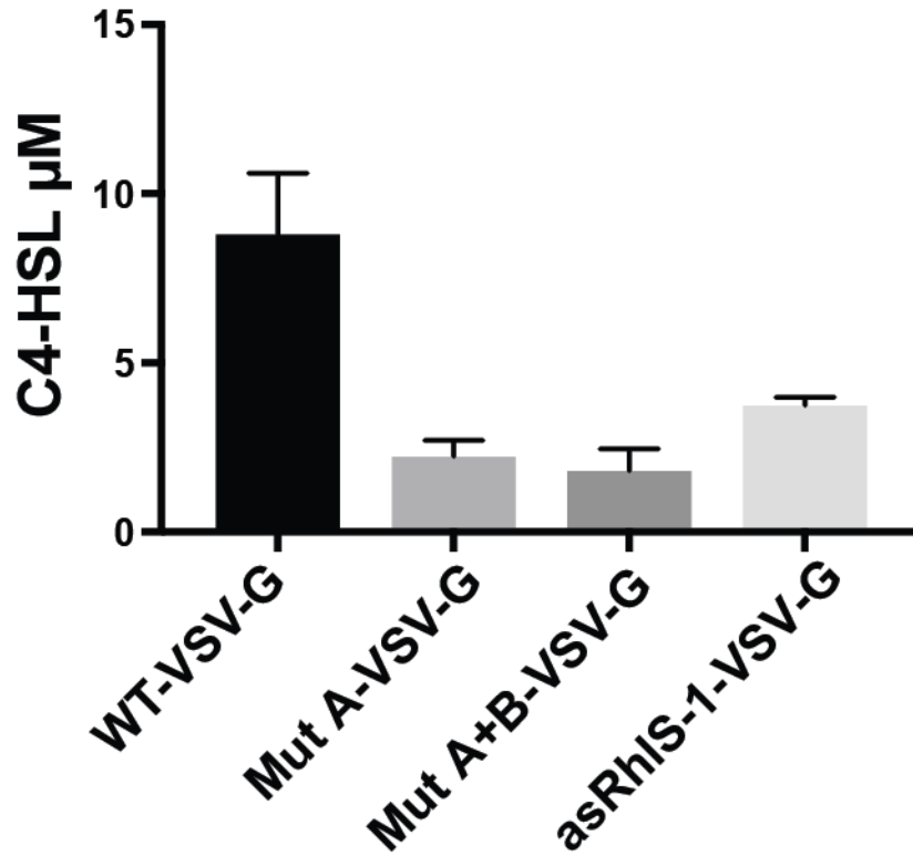
Figure S5: The RhII-VSV-G epitope tag does not alter C4-HSL production. Single colonies of WT RhII-VSV-G (MPK0698), RhIS Mut A-VSV-G (MPK0689), RhIS Mut A+B VSV-G (MPK0697) and the asRhIS-1-VSV-G (MPK0687) strains were grown for 24 h in 10 mL LB + 50mM MOPS in 50 mL flasks at 37°C with shaking. C4-HSL was measured as described in Fig 4B. Data are from three biological and two technical replicates for each strain and error bars are standard deviations.
