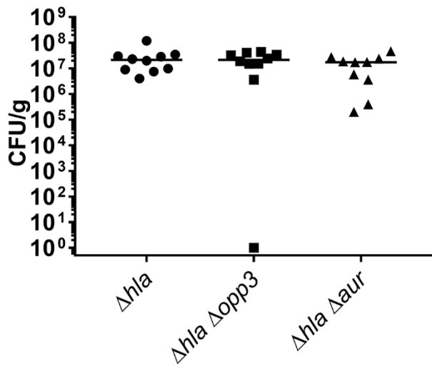
Figure S4. Bacterial burdens of 7-week old C57BL/6 mice subcutaneously infected with 1 \times 10^6 CFU of S. aureus \Delta hla , \Delta hla \Delta opp3 , or \Delta hla \Delta aur 5 days post infection. No statistical significance between the strains as determined by Kruskal-Wallis Test, n=10. Data are representative of 2 independent studies.
